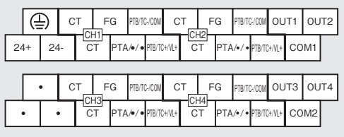
FX3U-4LC
