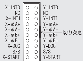
FX3U-20SSC-H
